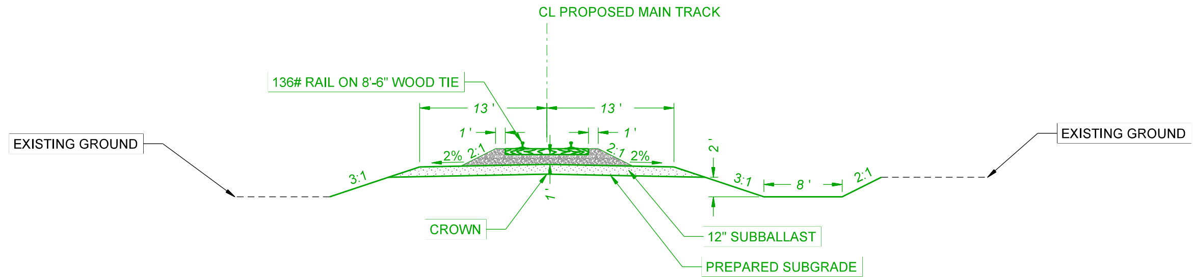
TYPICAL SECTION - SINGLE TRACK
